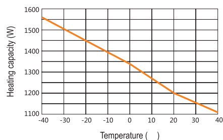
Heating capacity / Ambient temperature diagram
