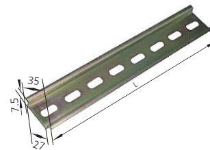
Mounting Rail Dimensions
