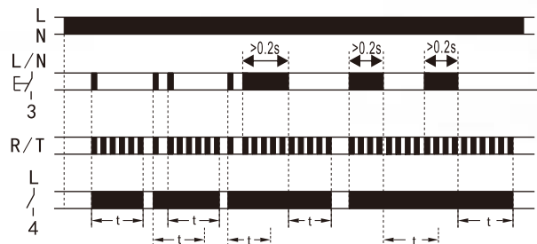
□ Function diagram
