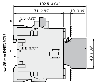
AF12 + VEM4 mechanical and electrical interlock set
