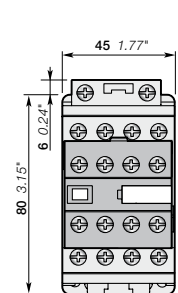
AF12 + CA4 4-pole auxiliary contact block
