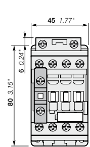
AF12 + CA4, CC4 1-pole auxiliary contact block
