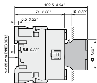
AF12 + CAT4 2-pole auxiliary contact and coil terminal block
