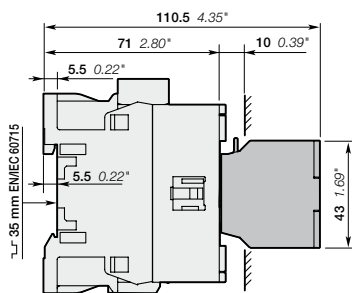
AF12 + CA4 4-pole auxiliary contact block
